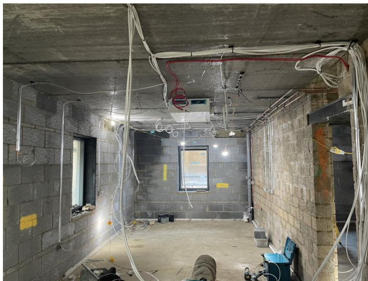
Ventilation system installation and 1st fix electric works to cluster kitchen in Preedy
