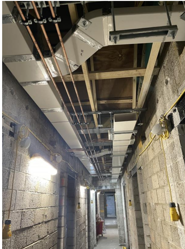
Ventilation ducts installed in cluster apartment corridor of Preedy
